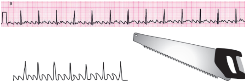
Fig. 8.25: Flutter auricular
