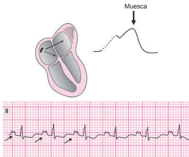
Fig. 7.11: P Mitral
